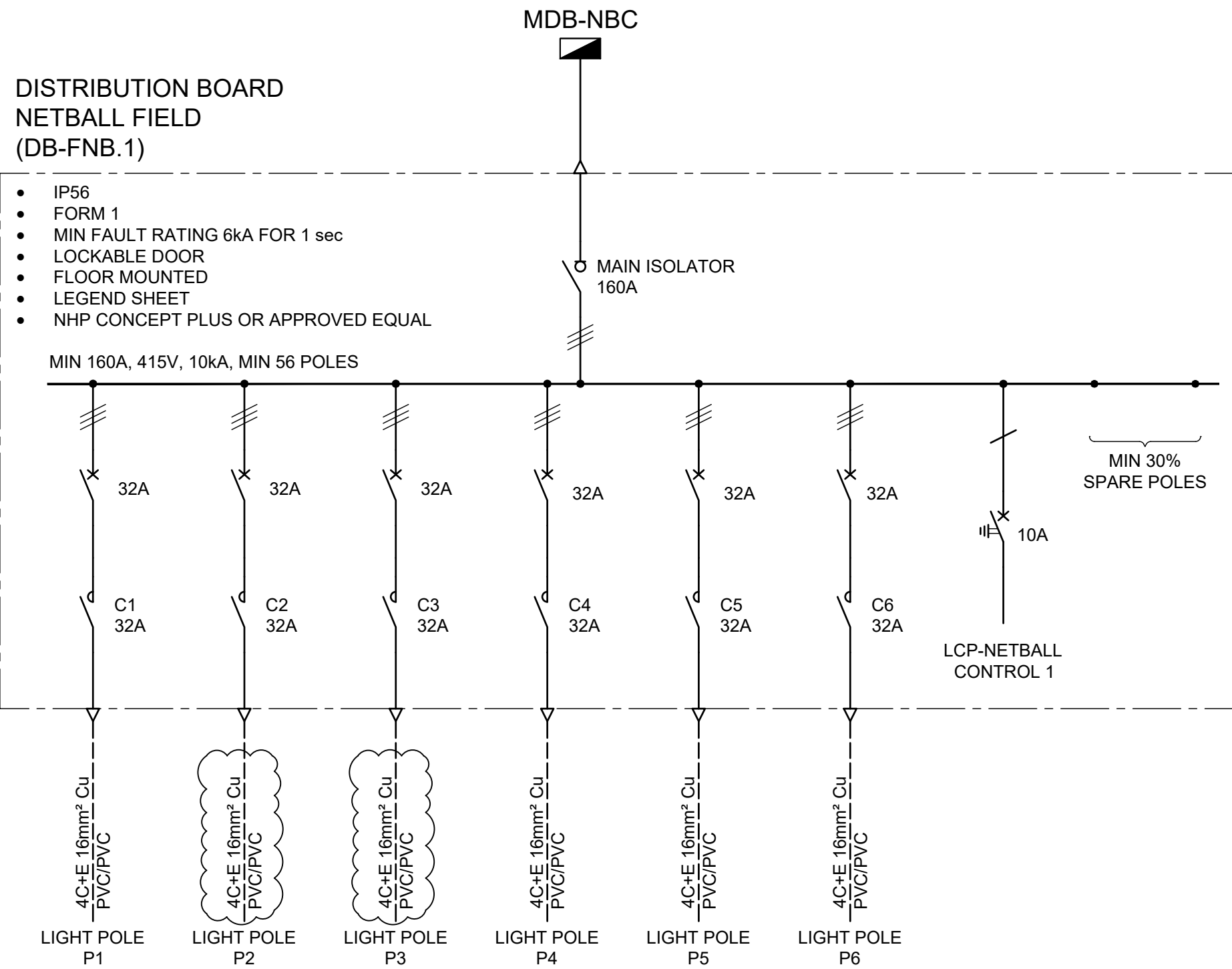
NETBALL FIELD DISTRIBUTION BOARD SLD (DB-FNB.1) NTS
