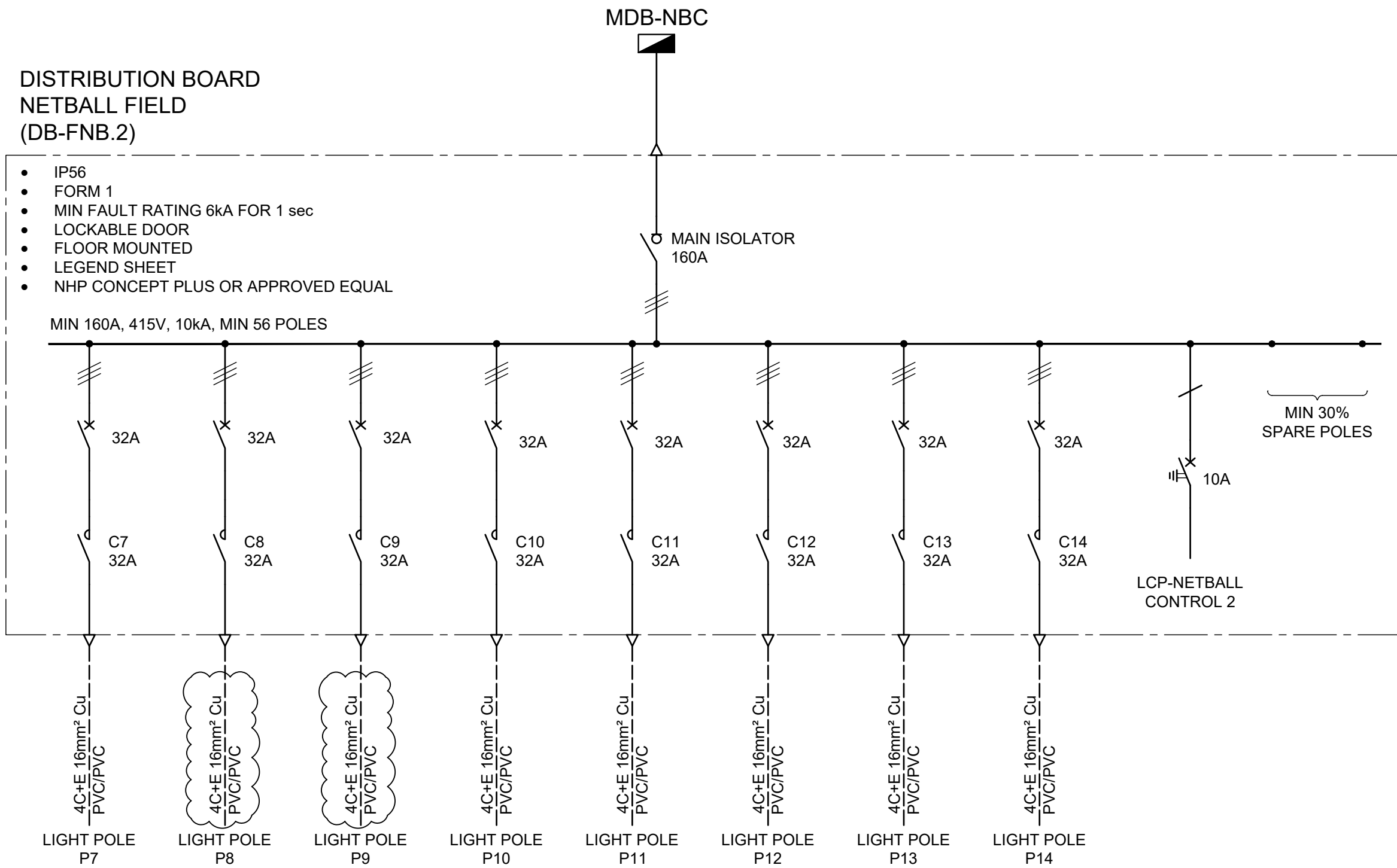
NETBALL FIELD DISTRIBUTION BOARD SLD (DB-FNB.2) NTS
