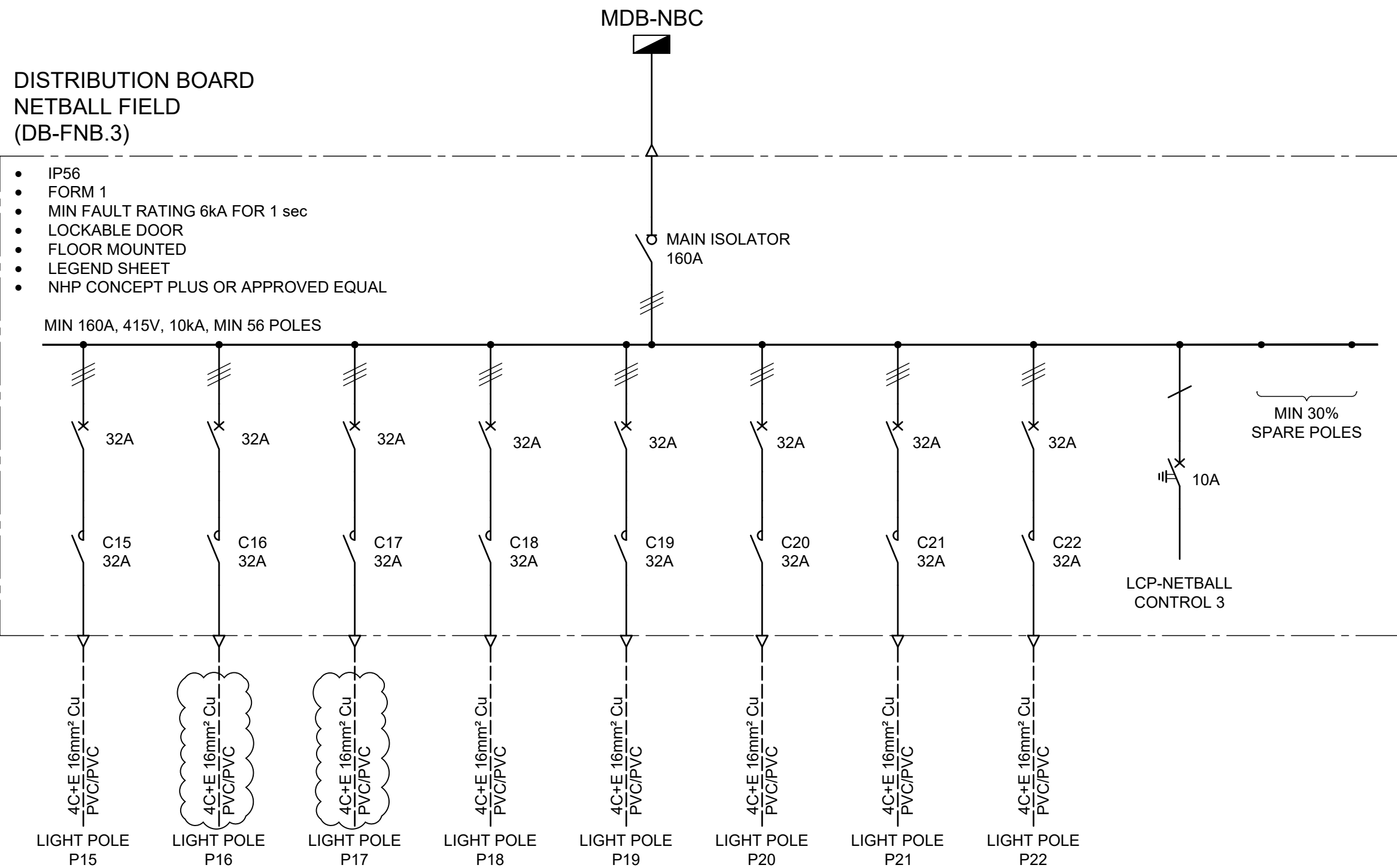
NETBALL FIELD DISTRIBUTION BOARD SLD (DB-FNB.3) NTS
